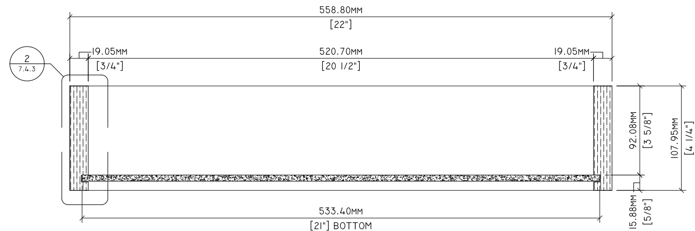
3 SECTION 7.4.2 3" = 1'-0"
