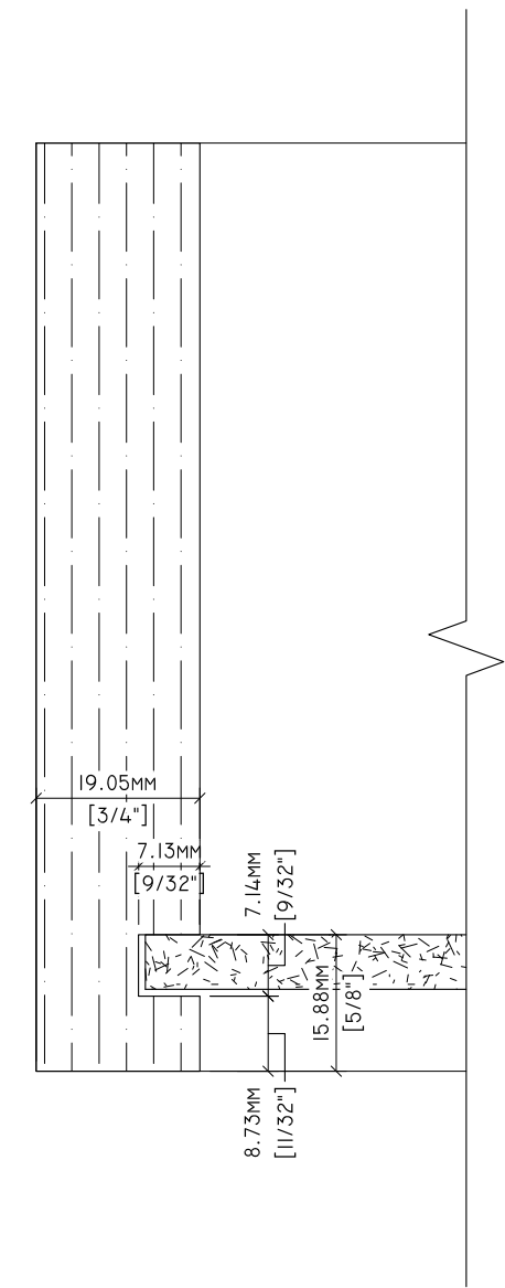
2 7.4.3 12" = 1'-0"
