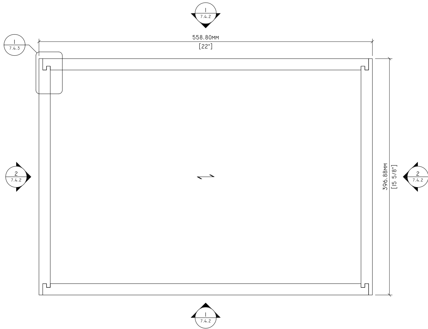
1 7.4.1 PLAN 3" = 1'-0"
