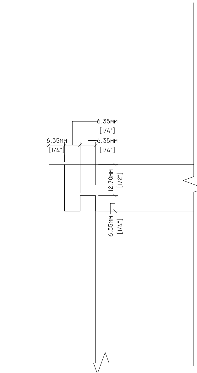
1 7.4.3 12" = 1'-0"
