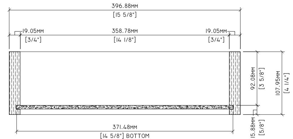
4 SECTION 7.4.2 3" = 1'-0"
