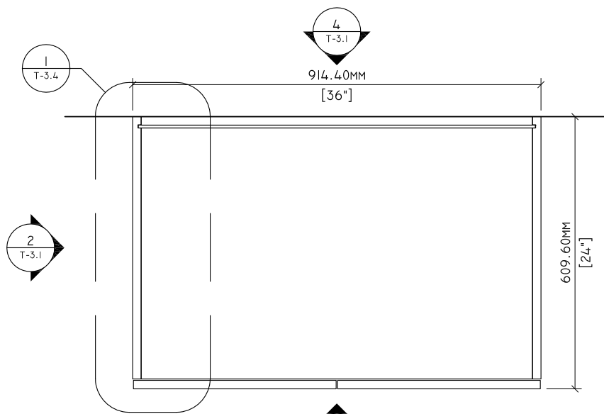
1 PLAN T-3.1 1" = 1'-0"
