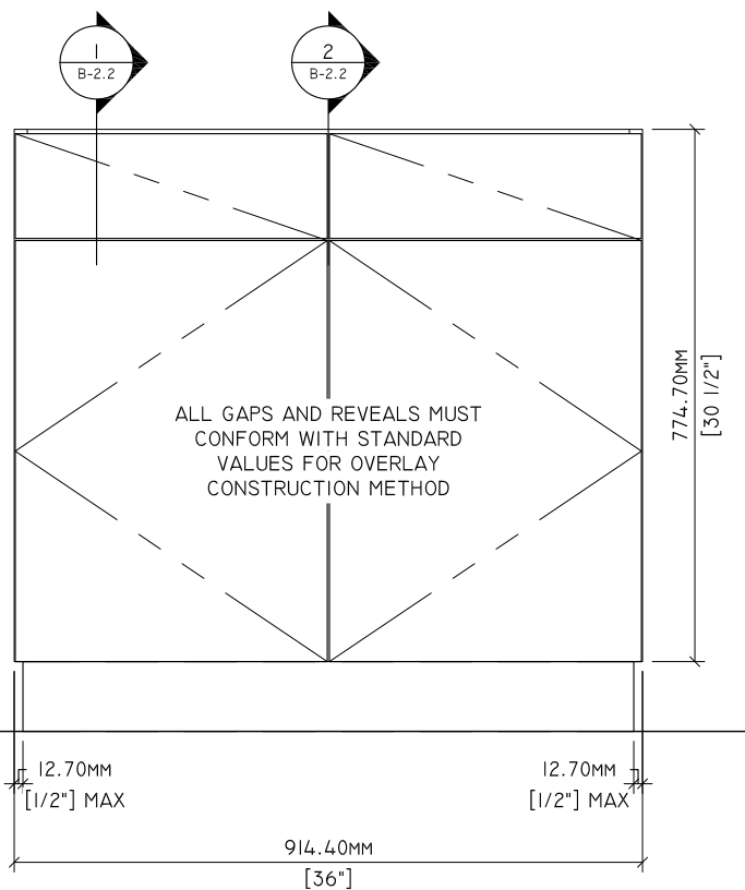
3 ELEVATION B-2.1 1" = 1'-0"
