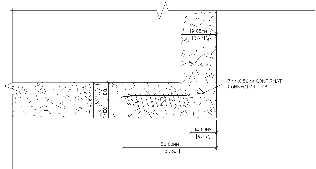
2 DETAIL T-2.4 12" = 1'-0"
